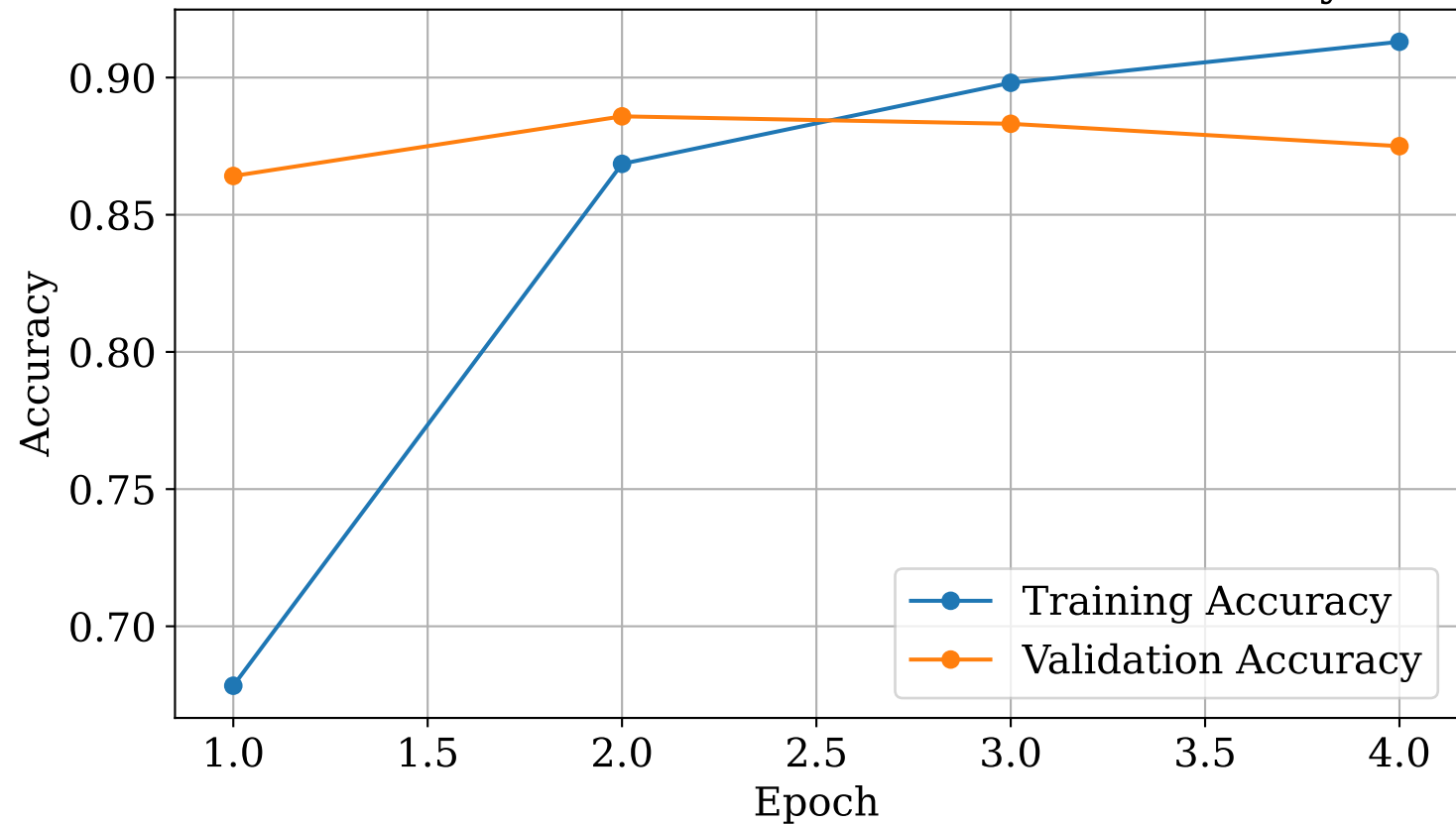
MobileNetV2 Feature Extraction - Accuracy
